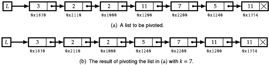
Figure 8.11: List pivoting.
