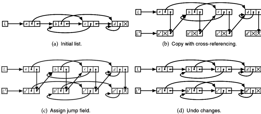
Figure 25.2: Duplicating a postings list.
