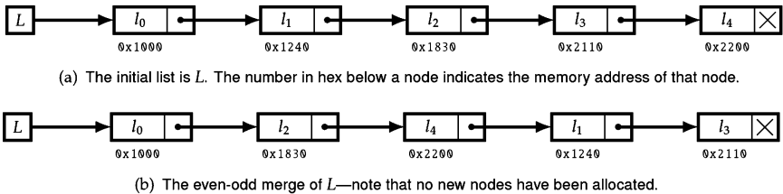
Figure 8.10: Even-odd merge example.
