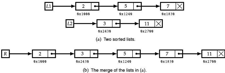
Figure 8.3: Merging sorted lists.
