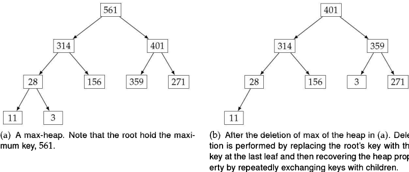
Figure 11.1: A max-heap and deletion on that max-heap.
