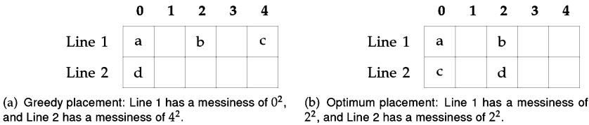
Figure 17.13: Assuming the text is “a b c d” and the line length is 5, placing words greedily results in a total messiness of 16, as seen in (a), whereas the optimum placement has a total messiness of 8, as seen in (b).
