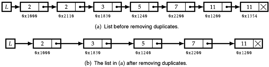
Figure 8.8: Example of duplicate removal.
