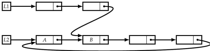
Figure 8.7: Overlapping lists.
