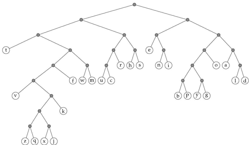
Figure 25.8: A Huffman tree for the English characters, assuming the frequencies given in Table 25.1 on the facing page.
