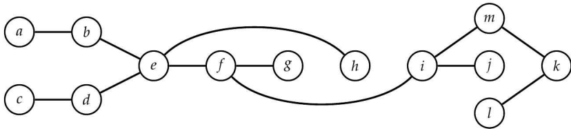
Figure 19.4: A tree.
