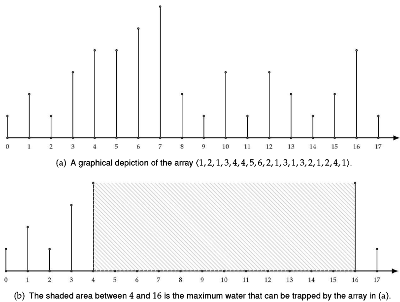
Figure 18.4: Example of maximum water trapped by a pair of vertical lines.
