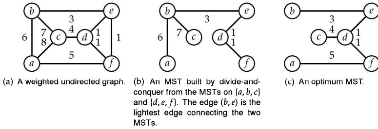
Figure 19.9: Divide-and-conquer applied to the MST problem is suboptimum—the MST in (b) has weight 18, but the MST in (c) has weight 14.
