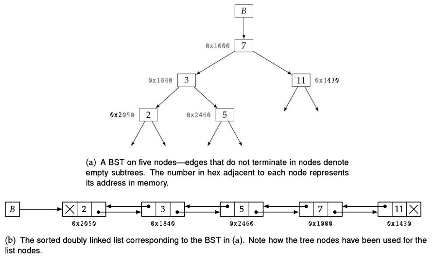
Figure 25.4: BST and sorted doubly linked list interconversion.
